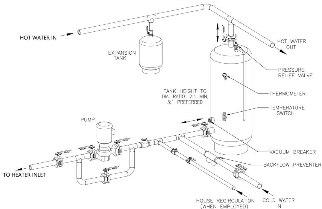
Figure 1: Stratified Storage Tank Piping Diagram
