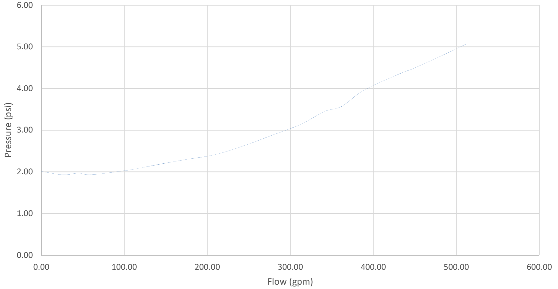
BMK4000/5000N \Delta Pressure (psi)
