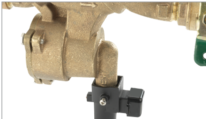
3. Ensure the sensor interface points in the same direction as the valve flow arrow.
