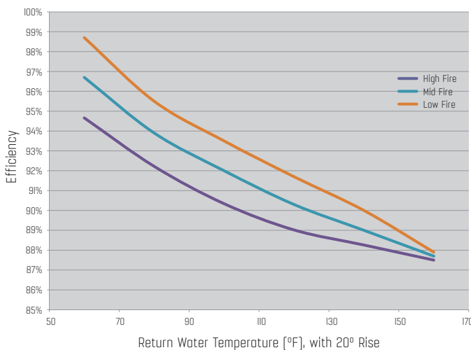
Efficiency of Modulex 450 to 1100
